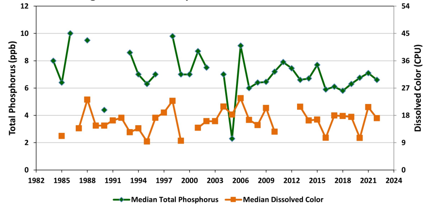
Figure 5. Bow Lake - Site 1 Ledges (1984-2022) Long-term Total Phosphorus and Dissolved Color Data
