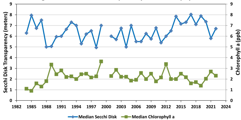
Figure 4. Bow Lake - Site 1 Ledges (1984-2022) Long-term Secchi Disk Transparency and Chlorophyll a Data
