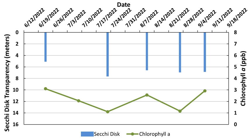
Figure 2. Bow Lake - 1 Ledges (2022 Seasonal Data) Secchi Disk Transparency and Chlorophyll a Data
