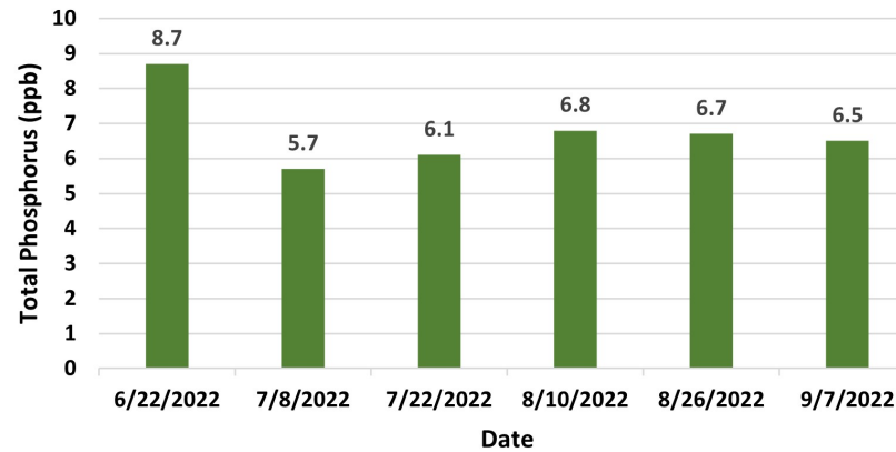
Figure 8. Bow Lake - Site 1 Ledges Surface Water Total Phosphorus Results
