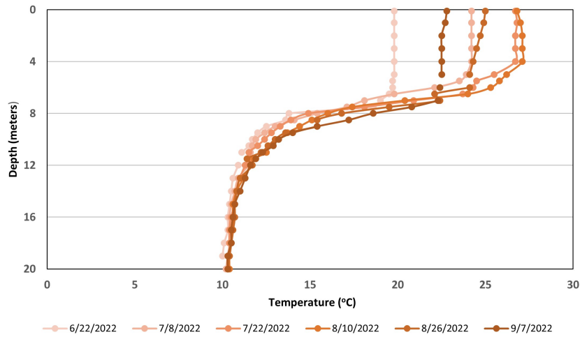
Figure 6. Bow Lake - Site 1 Ledges Temperature Profiles (June 22 through September 7, 2022)
