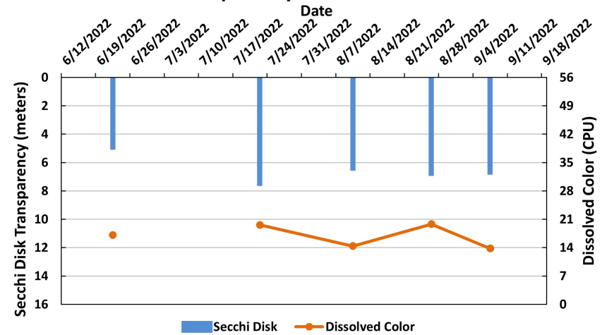
Figure 3. Bow Lake - 1 Ledges (2022 Seasonal Data) Secchi Disk Transparency and Dissolved Color Data
